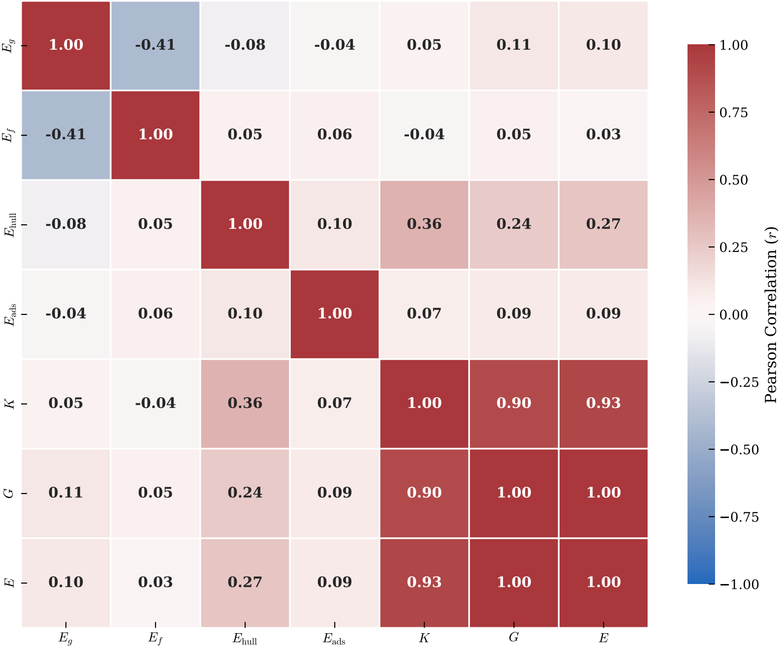
Inter-Property Correlation Matrix (Pearson r )
